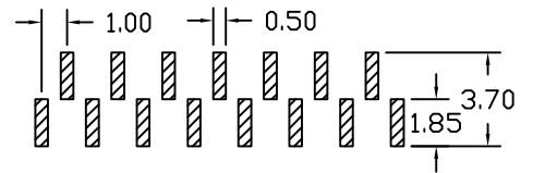
PCB LAYOUT
