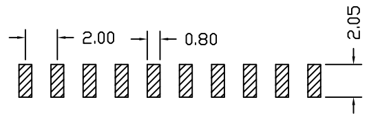
PCB LAYOUT
