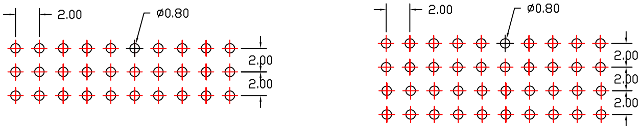
PCB LAYOUT
