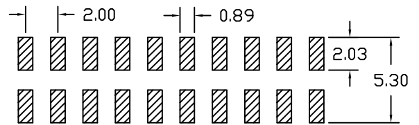
PCB LAYOUT
