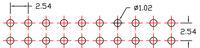
PCB LAYOUT
