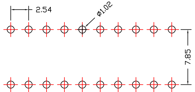
PCB LAYOUT
