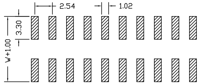
PCB LAYOUT
