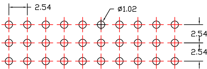
PCB LAYOUT
